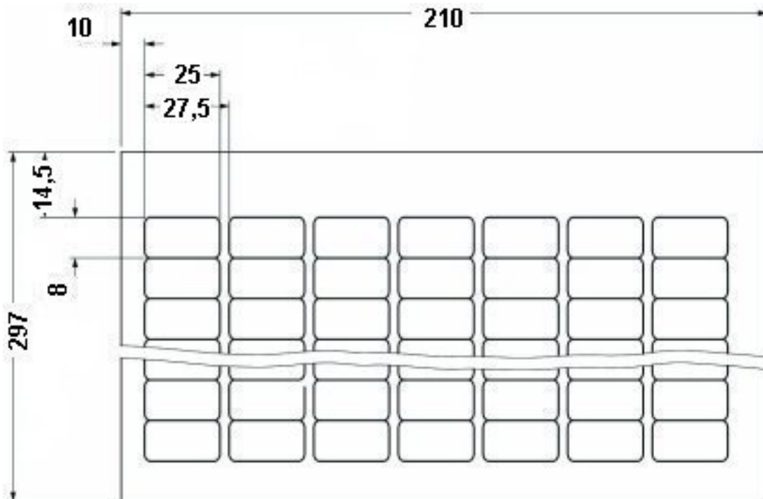
Dimensioned drawing
