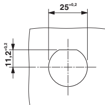
Dimensioned drawing
