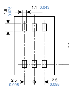
Recommended PC board pattern (TOP VIEW)
