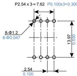
Recommended PC board pattern (TOP VIEW)
