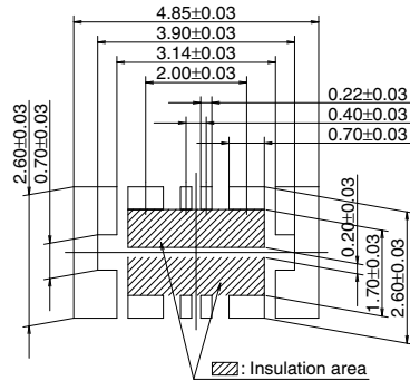
Recommended metal mask pattern
