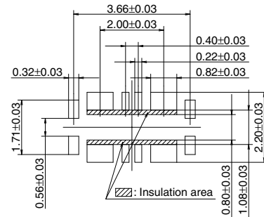
PC board pattern (TOP VIEW)
