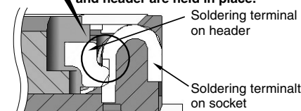
Cross section showing mating with soldering terminals
