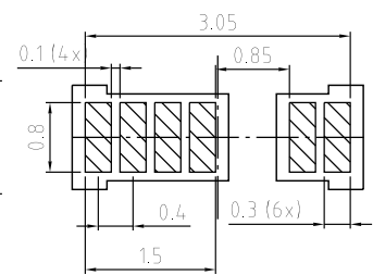
solder stencil
