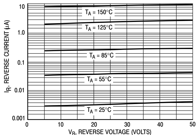
Figure 2. Leakage Current
