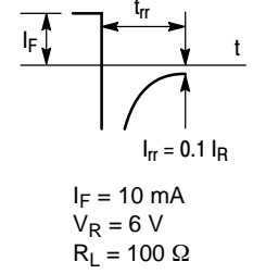
OUTPUT PULSE
