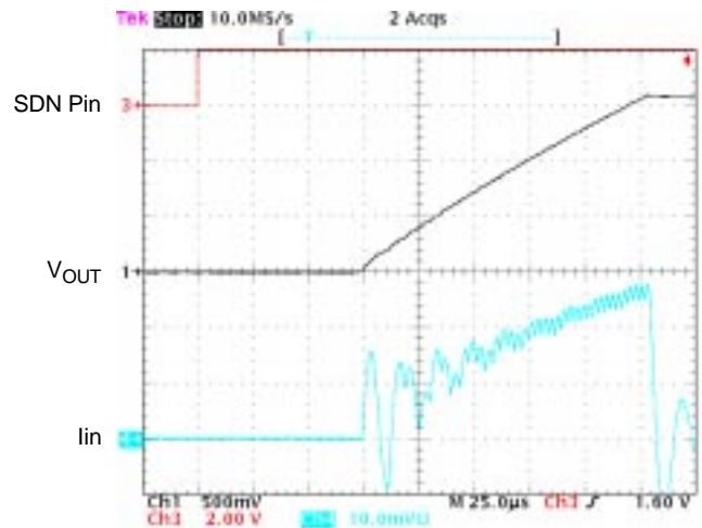
Figure 29. Pulse Startup Inrush Current – 400 Ω Load, 1.57 V out
