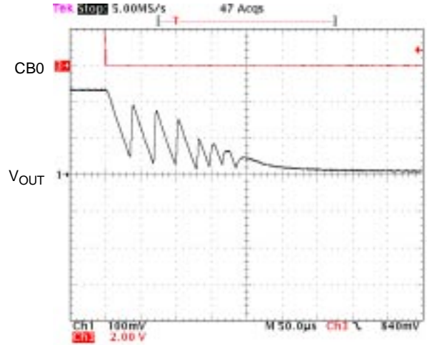
Figure 34. PWM DVM – 30 Ω Load, 1.35 to 1.57 V OUT
