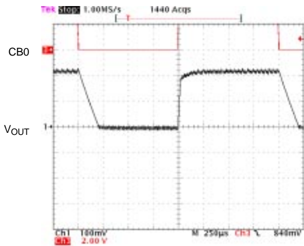
Figure 37. Pulse DVM – 150 Ω Load, 1.35 to 1.57 V OUT
