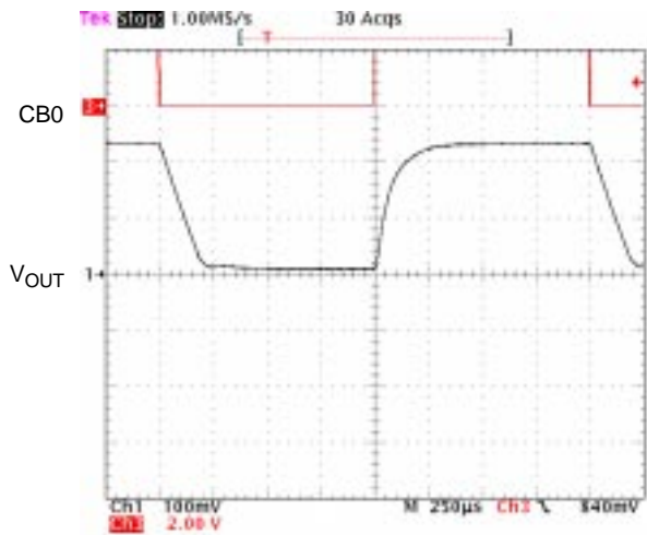
Figure 33. PWM DVM – 30 Ω Load, 1.35 to 1.57 V OUT
