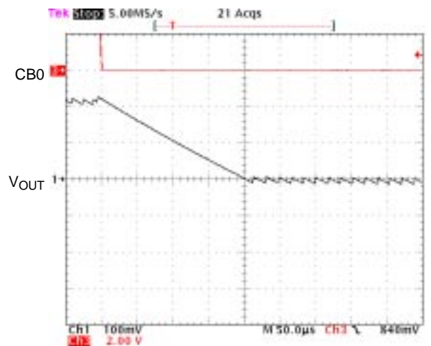
Figure 38. Pulse DVM – 150 Ω Load, 1.35 to 1.57 V OUT
