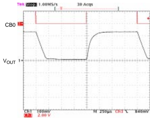
Figure 36. PWM DVM – 150 Ω Load, 1.35 to 1.57 V OUT
