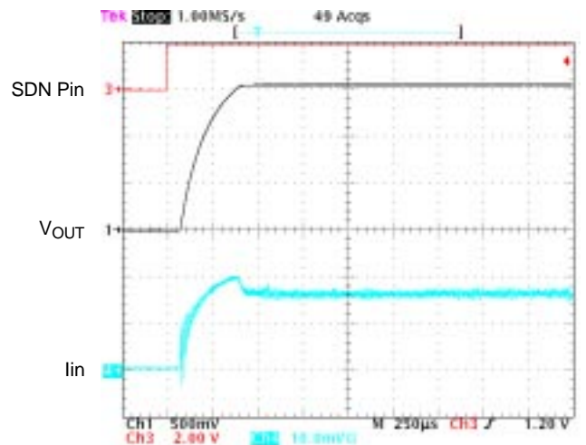
Figure 32. Pulse Startup Inrush Current – 25 Ω Load, 1.57 V out
