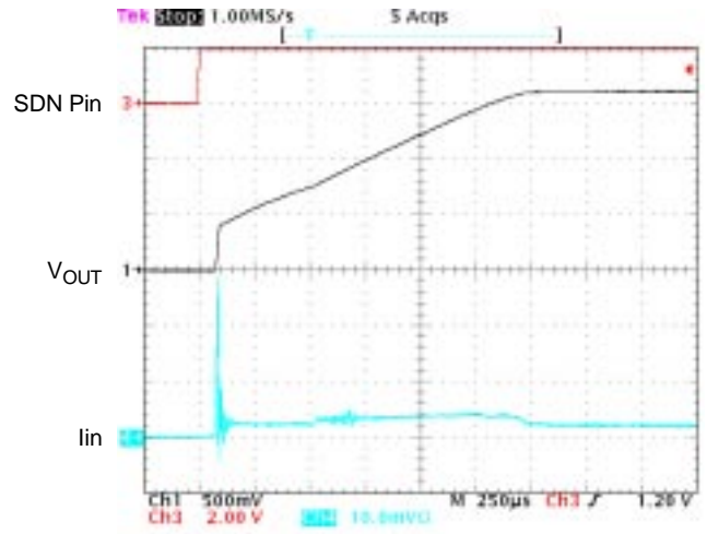
Figure 27. PWM Startup Inrush Current – 400 Ω Load, 1.57 V out
