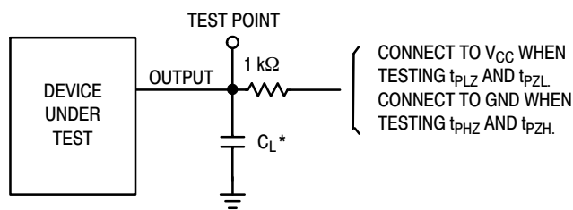
Figure 7. Test Circuit
