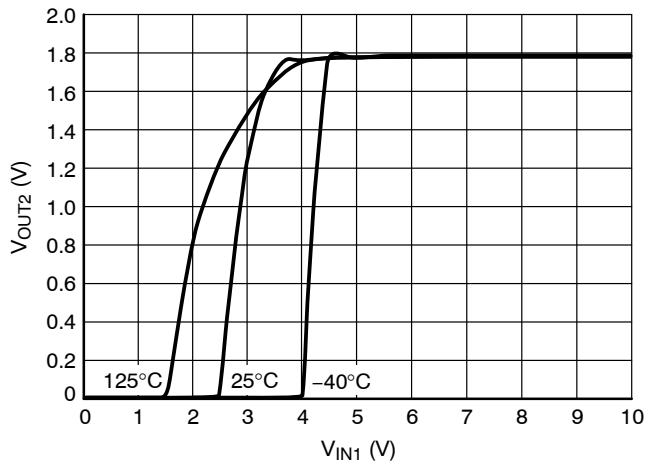
Figure 19. V_{OUT2} (1.8 V) versus V_{IN1}
