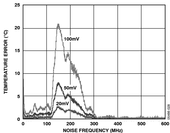
Figure 13. Temperature Error vs. Common-Mode Noise Frequency
