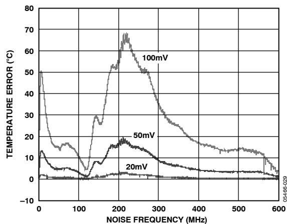
Figure 14. Temperature Error vs. Differential Mode Noise Frequency
