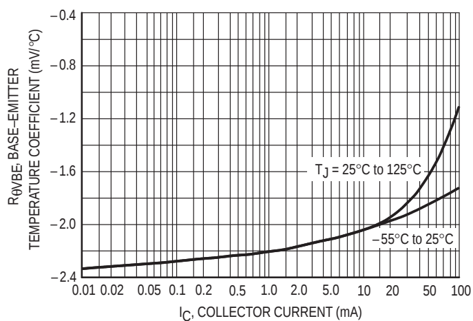
Figure 10. Temperature Coefficients
