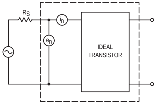
Figure 1. Transistor Noise Model
