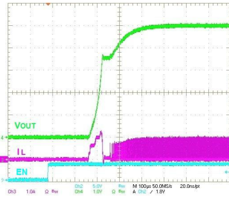
Figure 14. Startup, 50 \Omega Load
