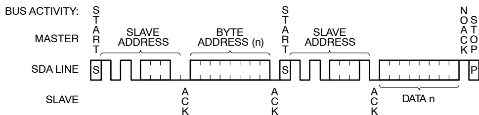
Figure 10. EEPROM Selective Read
