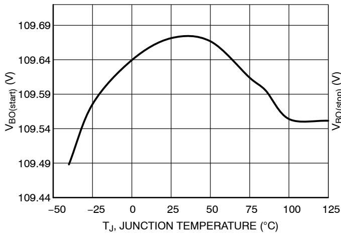
Figure 37. V_{\text{BO(start)}} vs. Temperature
