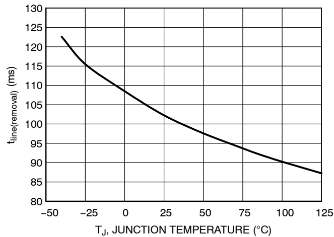
Figure 36. t_{\text{line(remove)}} vs. Temperature
