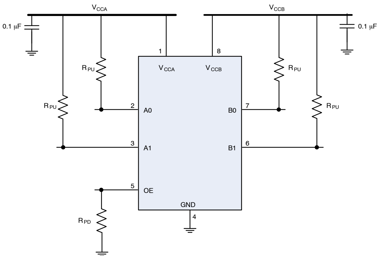
Figure 4. Application Circuit
