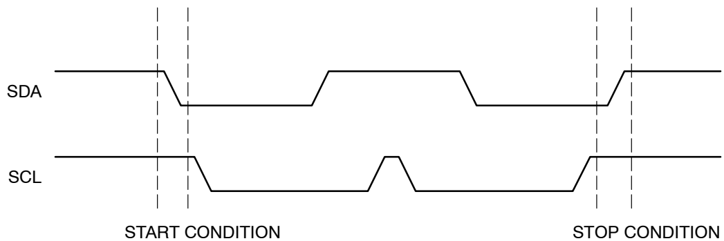
Figure 16. Start/Stop Condition
