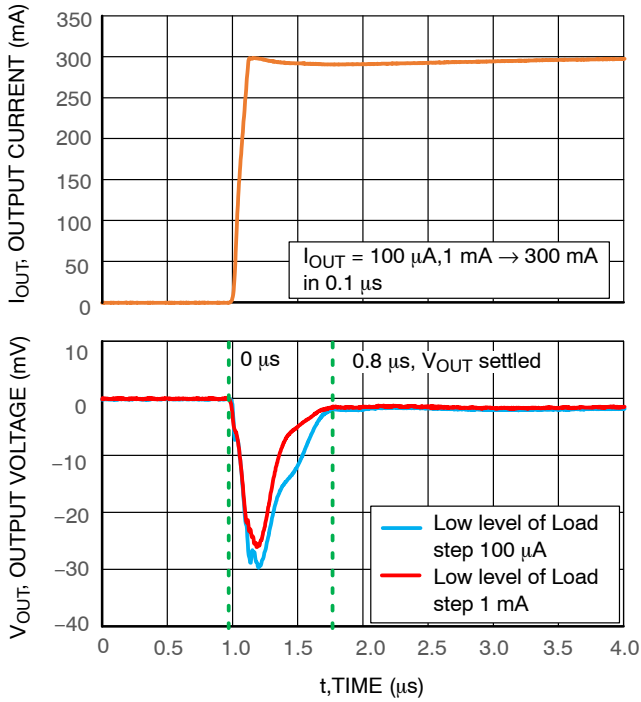
Figure 4. Load Transient Response for 0.1\text{ }\mu\text{s} Edge and Different Low Level of Load Step
