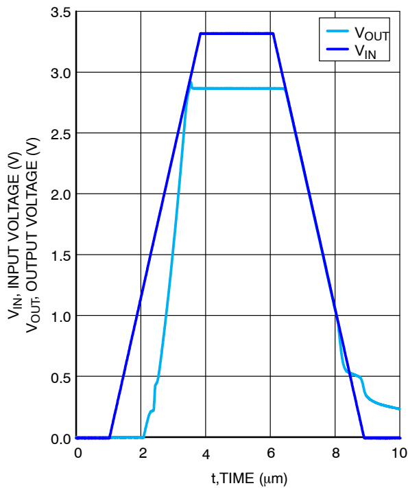
Figure 33. Turn On/Off – Slow Rising – V_{OUT(NOM)} = 2.85\text{ V}
