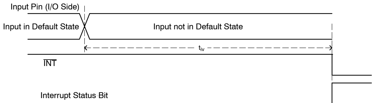
Figure 5. Time to INT from Change in Input Default State
