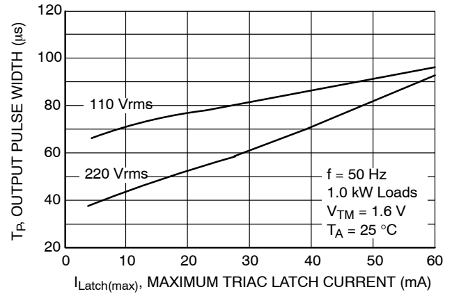
Figure 8. Output Pulse Width versus Maximum Triac Latch Current
