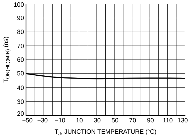
Figure 42. Minimum On Time @ V_{SENSE} = 2.8 V vs. Temperature
