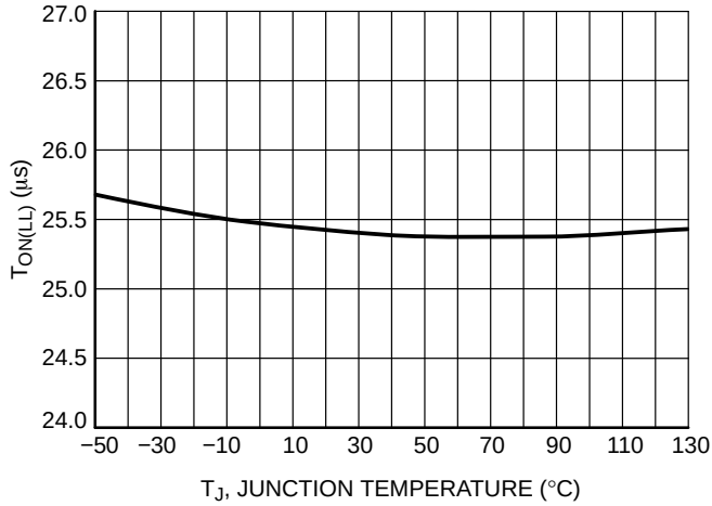
Figure 39. Maximum On Time @ V_{SENSE} = 1.4 V vs. Temperature
