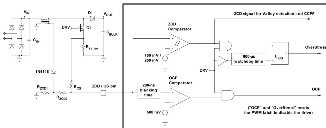
Figure 68. Current Sense and Zero Current Detection Blocks
