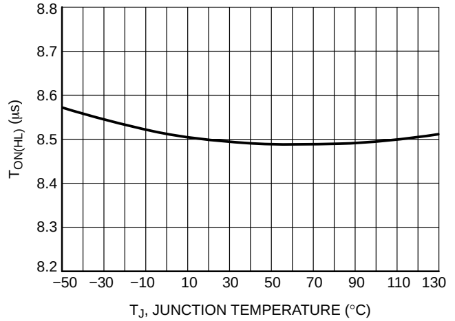
Figure 40. Maximum On Time @ V_{SENSE} = 2.8 V vs. Temperature
