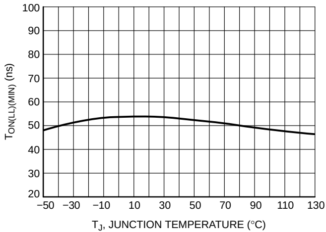
Figure 41. Minimum On Time @ V_{SENSE} = 1.4 V vs. Temperature
