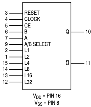
Figure 2. Block Diagram
