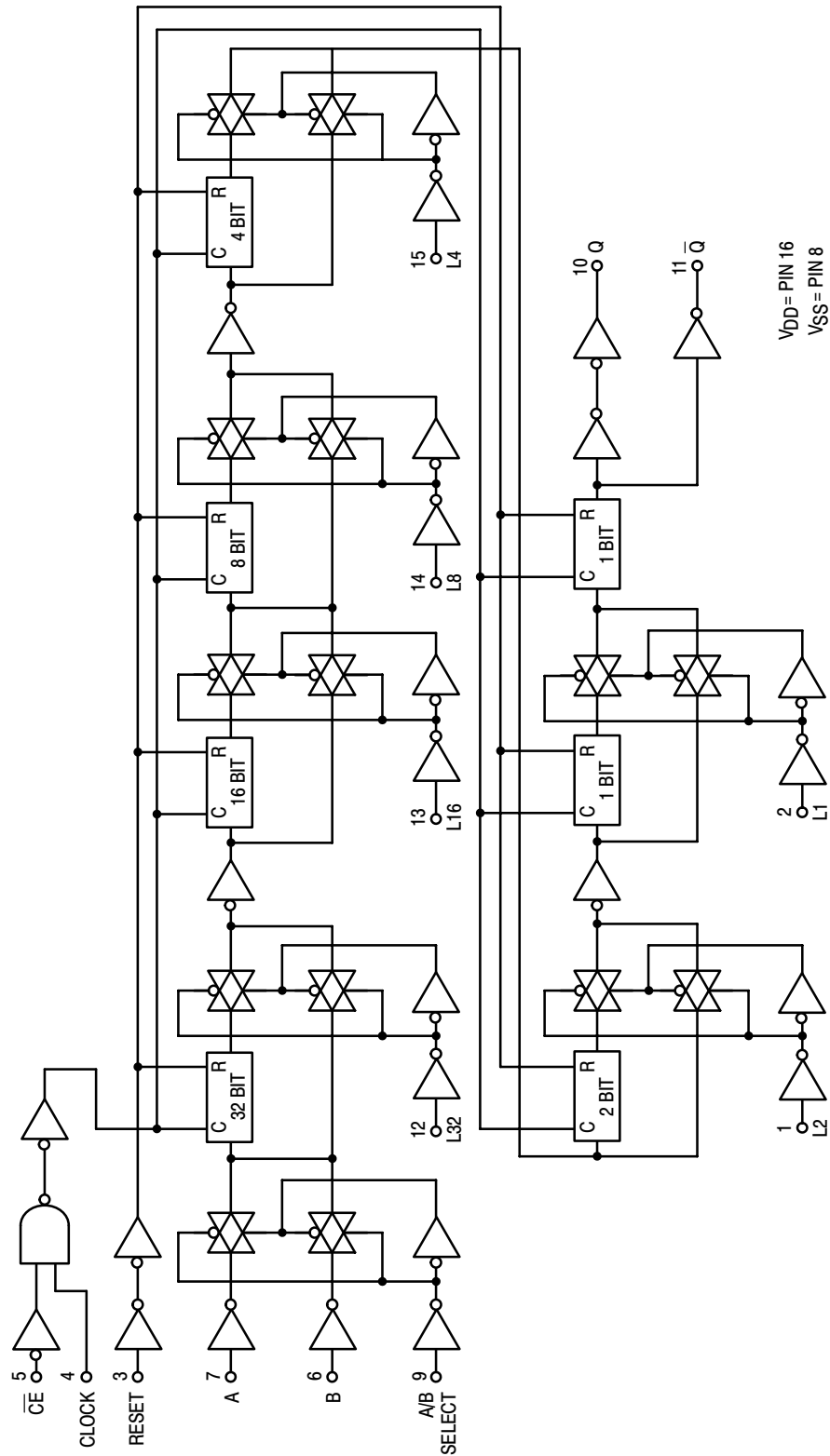
Figure 1. Logic Diagram
