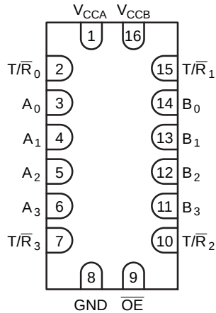
Figure 1. DQFN Pad Assignments (Top Through View)
