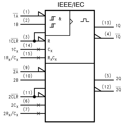
Figure 2. Logic Symbol
