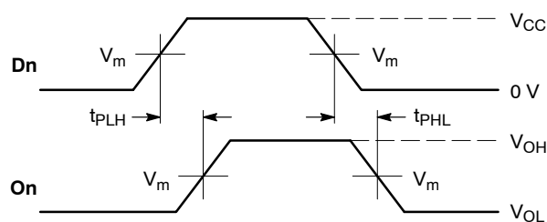
WAVEFORM 1 – PROPAGATION DELAYS
