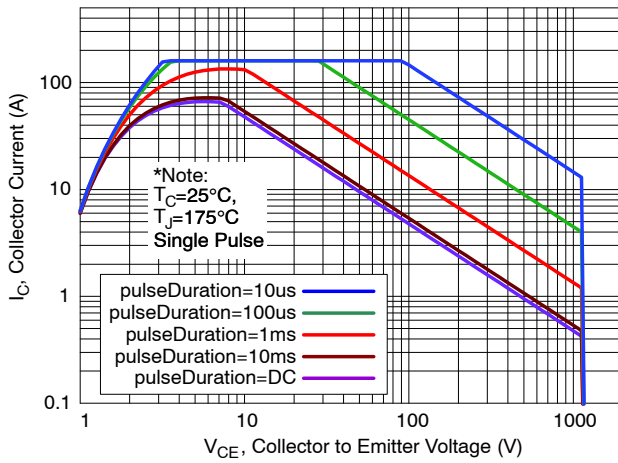
Figure 9. SOA Characteristics
