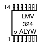
TSSOP-14
