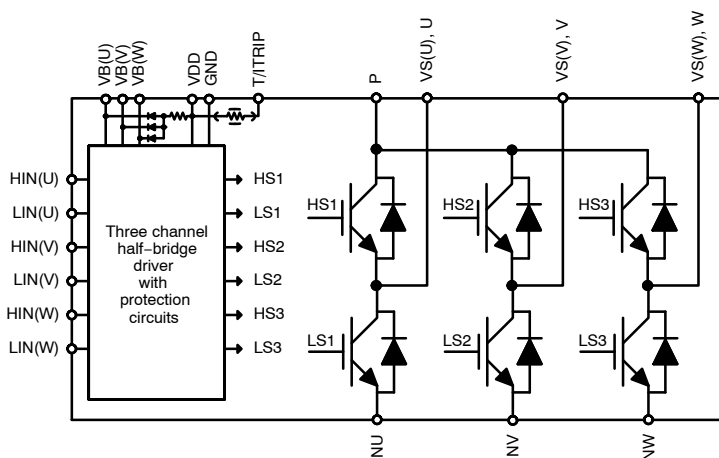
Figure 1. Functional Diagram
