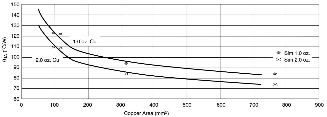
Figure 22. SOIC-14, \theta_{JA} as a Function of the Pad Copper Area Including Traces, Board Material
