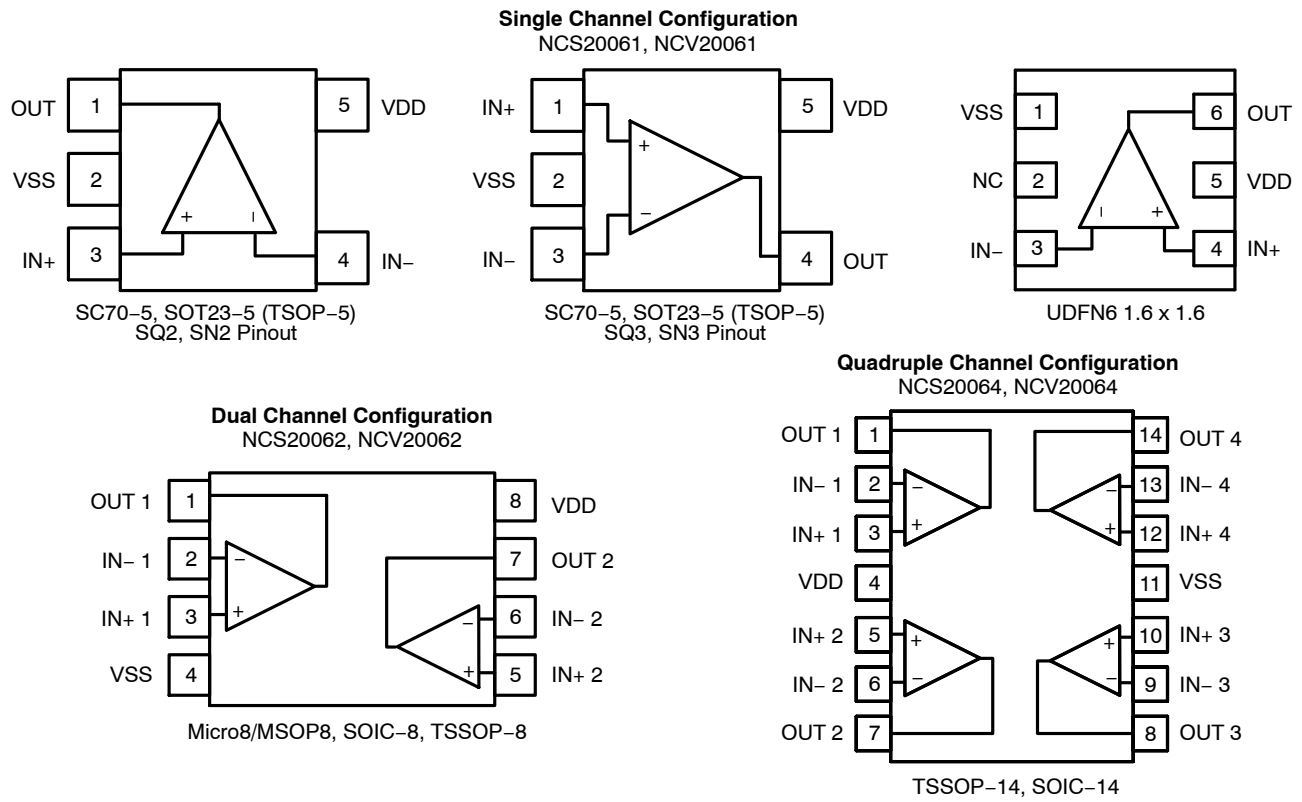
Figure 1. Pin Connections
