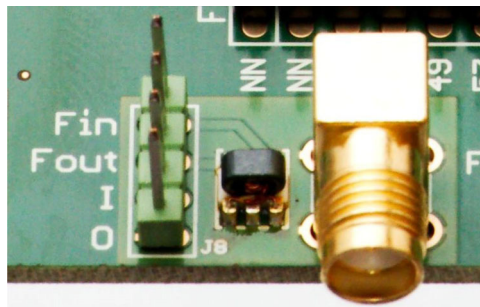
Figure 11. (right) photo and (left) schematic of the BOB SMA, balun transformer and 4-pin header arrangement.
