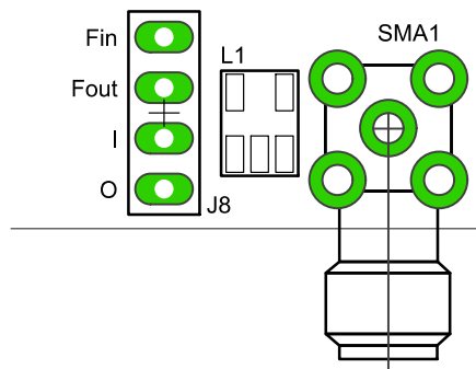
Figure 11. (right) photo and (left) schematic of the BOB SMA, balun transformer and 4-pin header arrangement.
