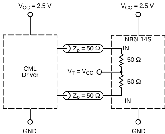
Figure 13. CML Interface
