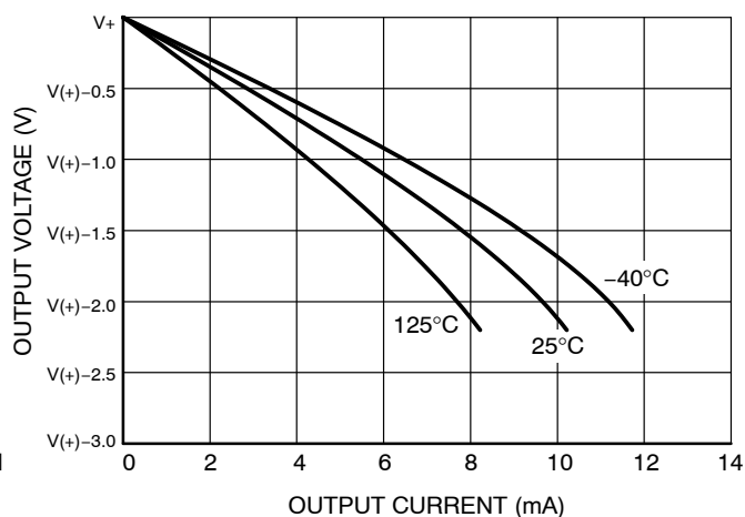
Figure 11. Positive Output Voltage Swing vs. Output Current, V_S = 2.2\text{ V}
