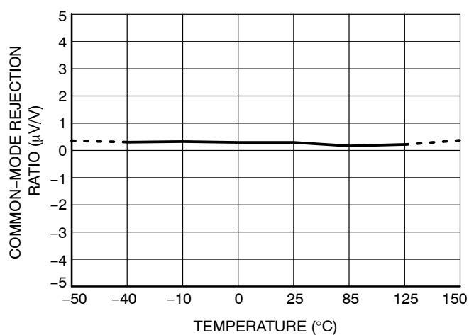
Figure 5. Common-Mode Rejection Ratio vs. Temperature
