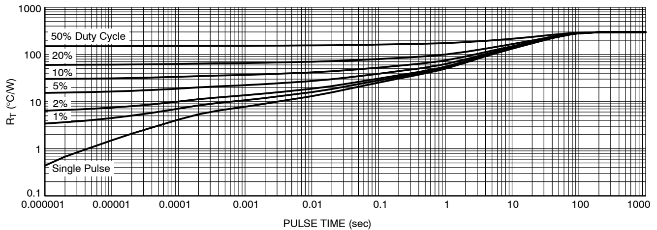
Figure 26. Thermal Response
