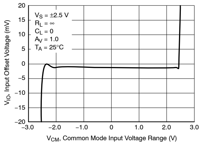
Figure 27. Input Offset Voltage vs. Common Mode Input Voltage Range V_S = \pm 2.5\text{ V}
