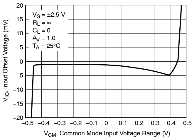
Figure 28. Input Offset Voltage vs. Common Mode Input Voltage Range, V_S = \pm 0.45\text{ V}
