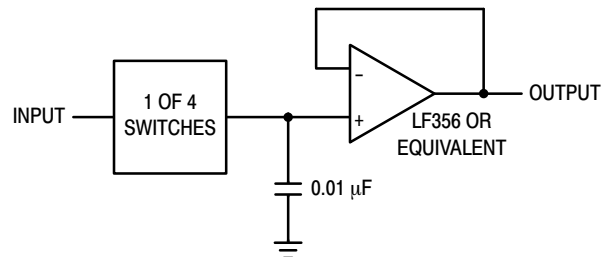
Figure 21. Sample/Hold Amplifier
