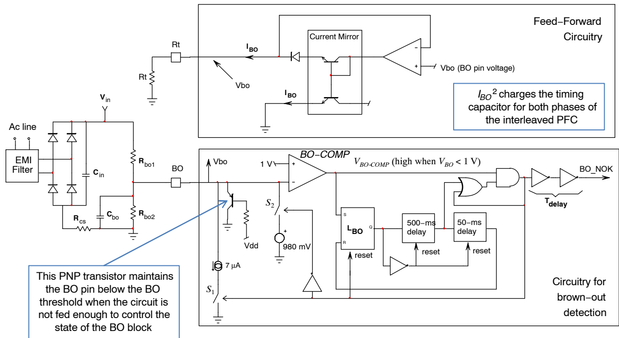
Figure 22. Brown-out Block
