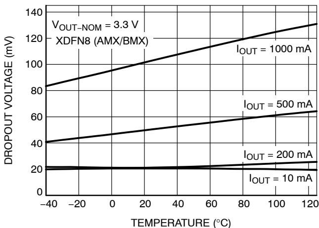
Figure 12. Dropout Voltage vs. Temperature
