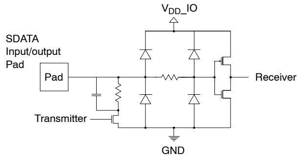
Figure 35. Serial Interface
