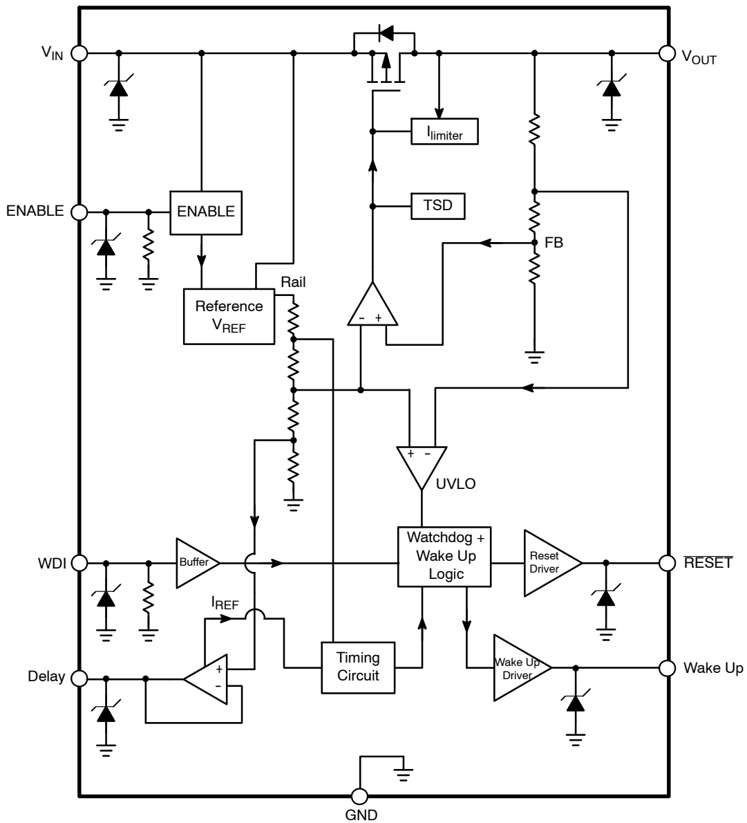
Figure 1. Block Diagram
