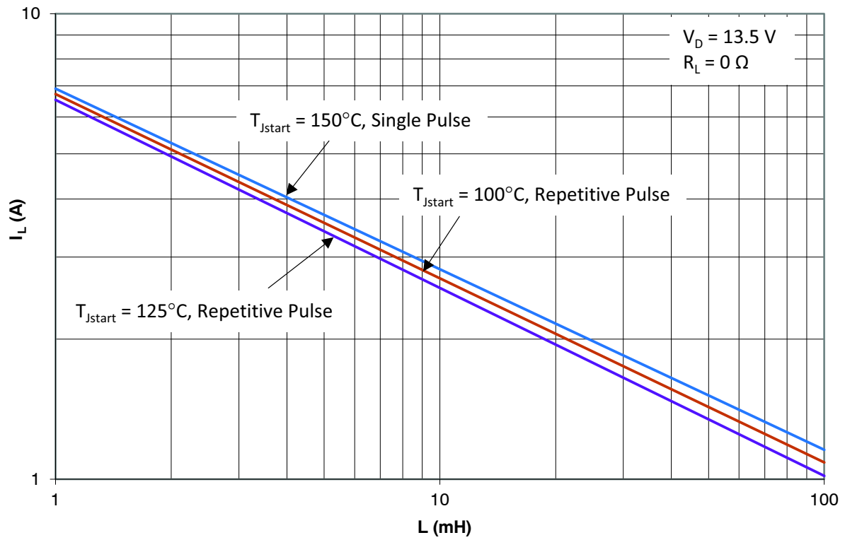
Figure 37. Maximum Switch-Off Current vs. Load Inductance, V_D = 13.5 V; R_L = 0 \Omega
