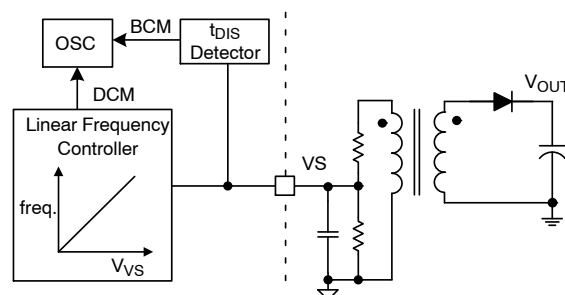
Figure 19. Linear Frequency Control
