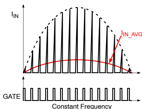
Figure 18. PFC Control in DCM
