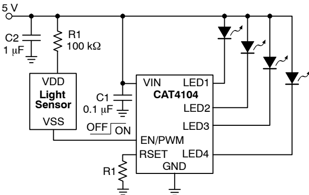
Figure 21. Daylight Detection
