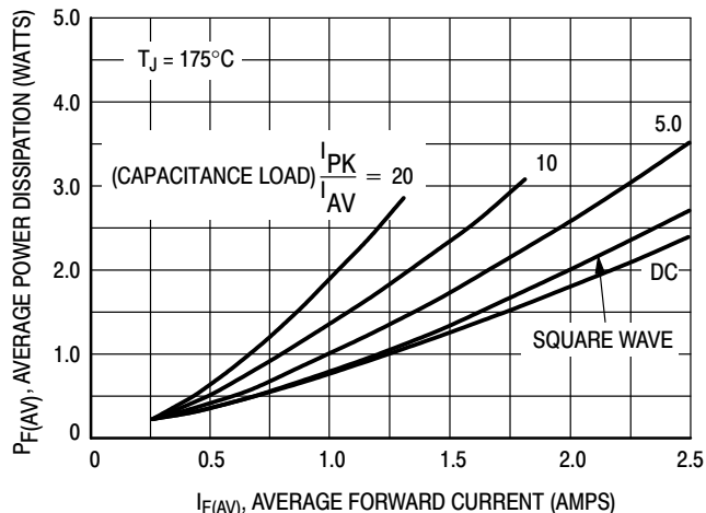
Figure 5. Power Dissipation
