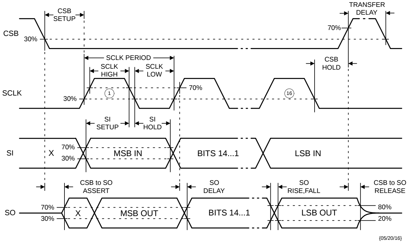
Figure 4. SPI Timing
