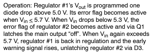
Figure 25. Regulator with Early Warning and Auxiliary Output
