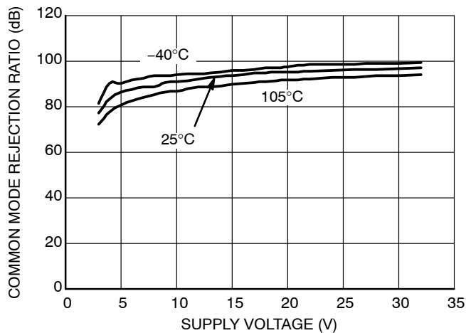
Figure 7. NCS1002A CMRR vs. Supply Voltage
