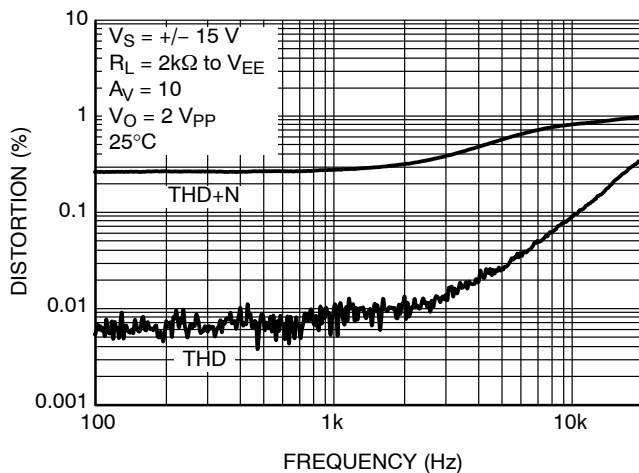
Figure 8. Distortion vs. Frequency
