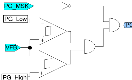
Figure 9. PG Block Diagram
