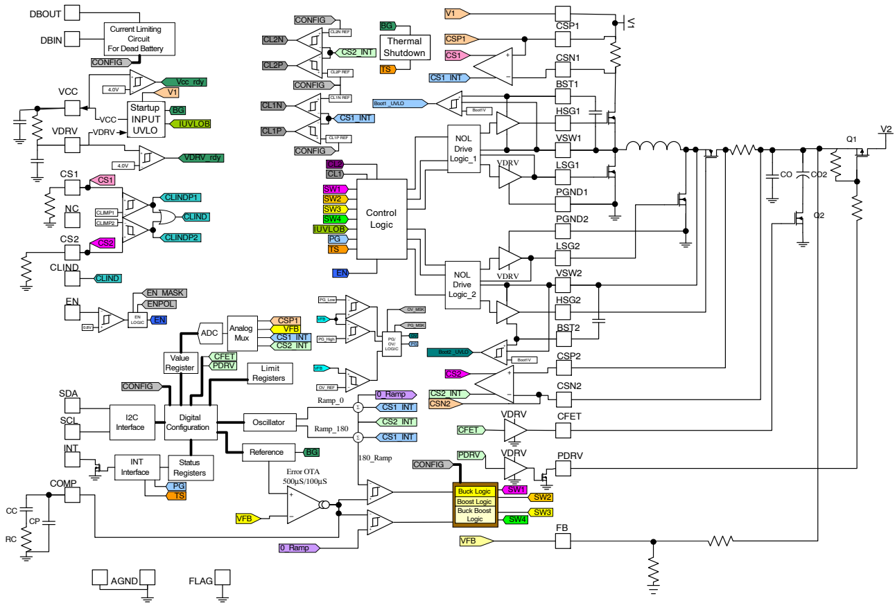
Figure 3. Block Diagram
