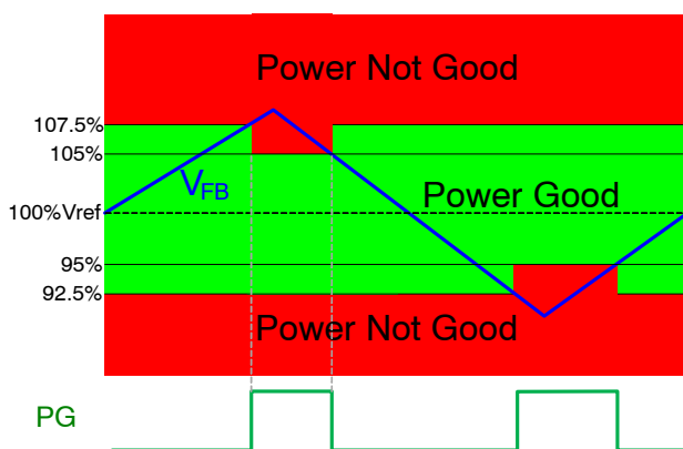
Figure 10. PG Diagram
