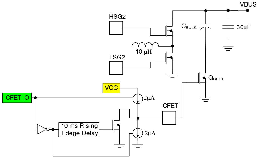
Figure 11. CFET Drive
