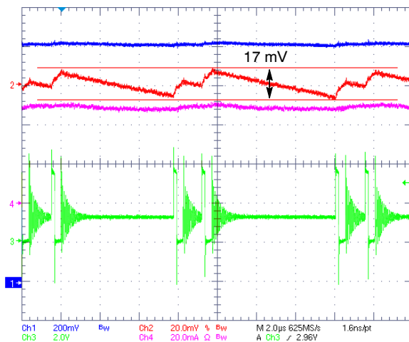
Figure 25. PFM Ripple
